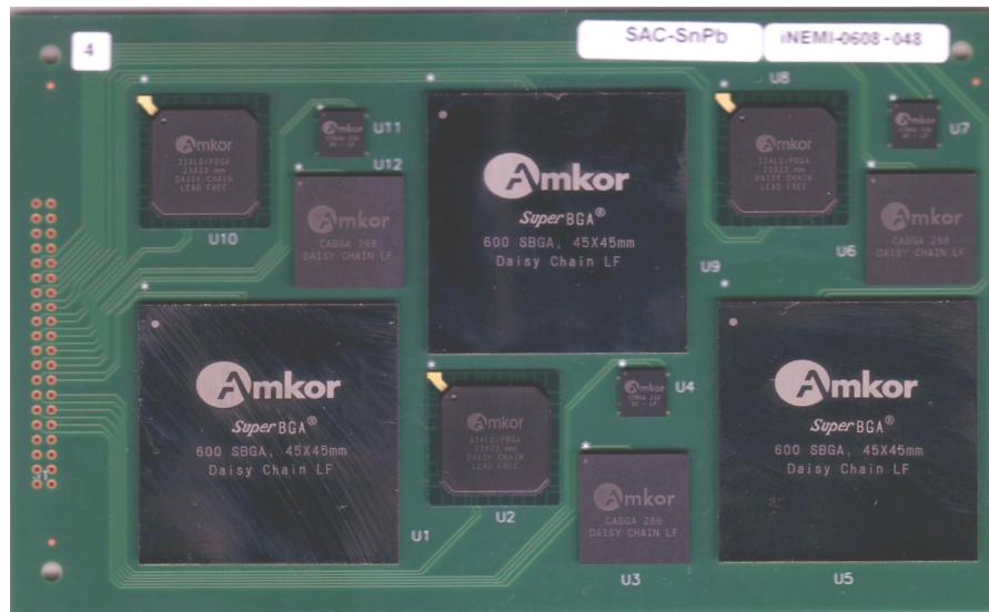
Figure 3: Representative assembled test board.
