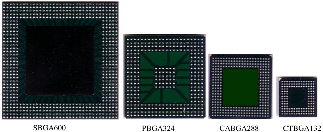
Figure 1: Components, ball side up
