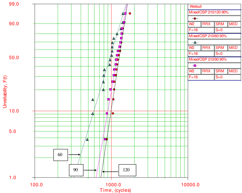
Figure 6: A Weibull plot showing the impact of the time above liquidus temperature on solder joint reliability for the CTBGA132 component.
