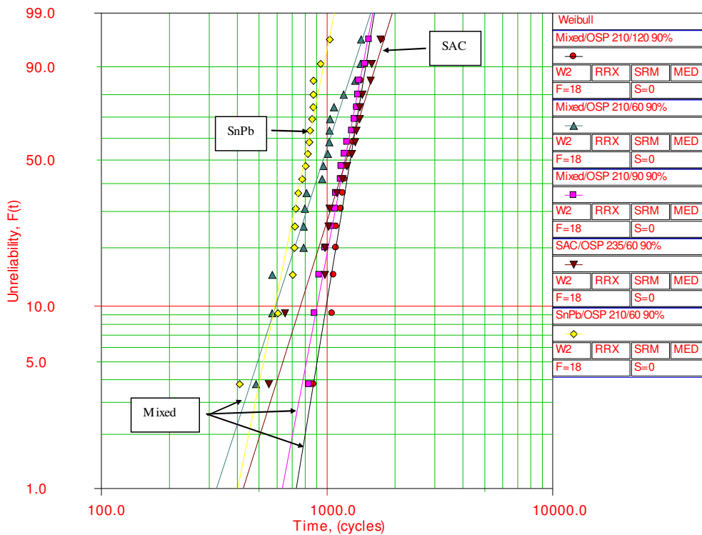
Figure 16: Weibull plot showing a comparison of the solder joint reliability between the mixed soldering conditions and the pure Sn-Pb and pure SAC soldering conditions on the CTBGA132 package.
