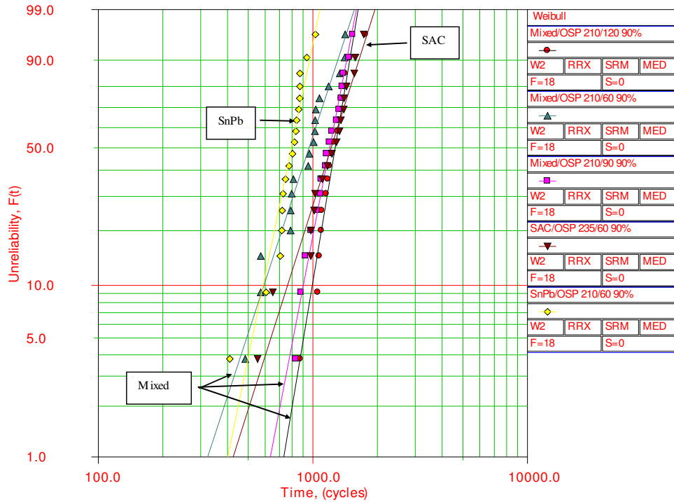
Figure 9: A Weibull plot showing the reliability of mixed alloy (Sn-Pb and Sn-Ag-Cu) solder joints, the “pure” Sn-Pb and “pure” Sn-Ag-Cu solder joints as a function of the time above liquidus for the CTBGA132 component.
